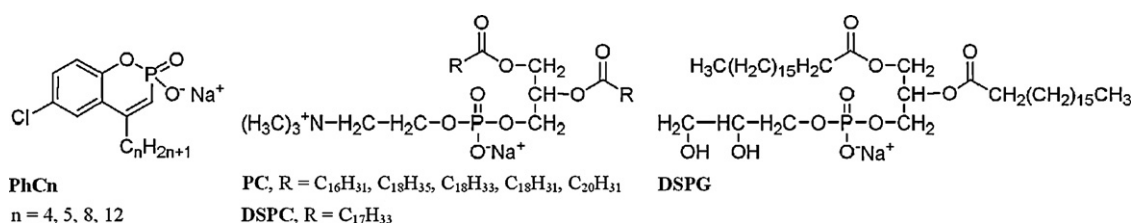
Scheme 2. Chemical structures of phosphocoumarines, DSPG, DSPC and PC.
