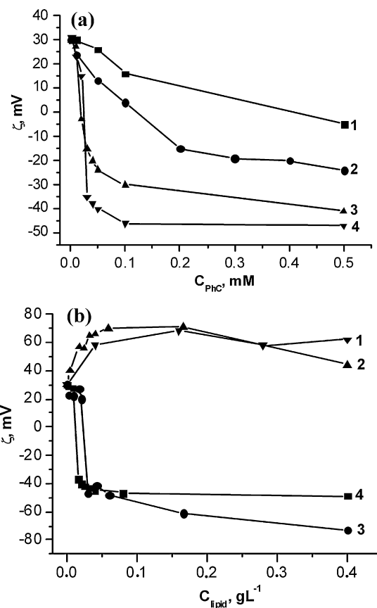
Fig. 1. The \xi -potential value of Tb(III) doped SNs ( C = 0.028 \text{g L}^{-1} ) at 0.01 mM of 16-6-16 and various amounts of (a): phosphacomarins PhC4 (1), PhC5 (2), PhC8 (3) and PhC12 (4) ( \text{SD} = 5 mV, n = 3 ) and (b): lipids DSPC (1) ( \text{SD} = 15 mV, n = 3 ), PC 99% (2) ( \text{SD} = 15 mV, n = 3 ), PC 60% (3) ( \text{SD} = 5 mV, n = 3 ) and DSPG (4) ( \text{SD} = 5 mV, n = 3 ) at pH 9.2.
