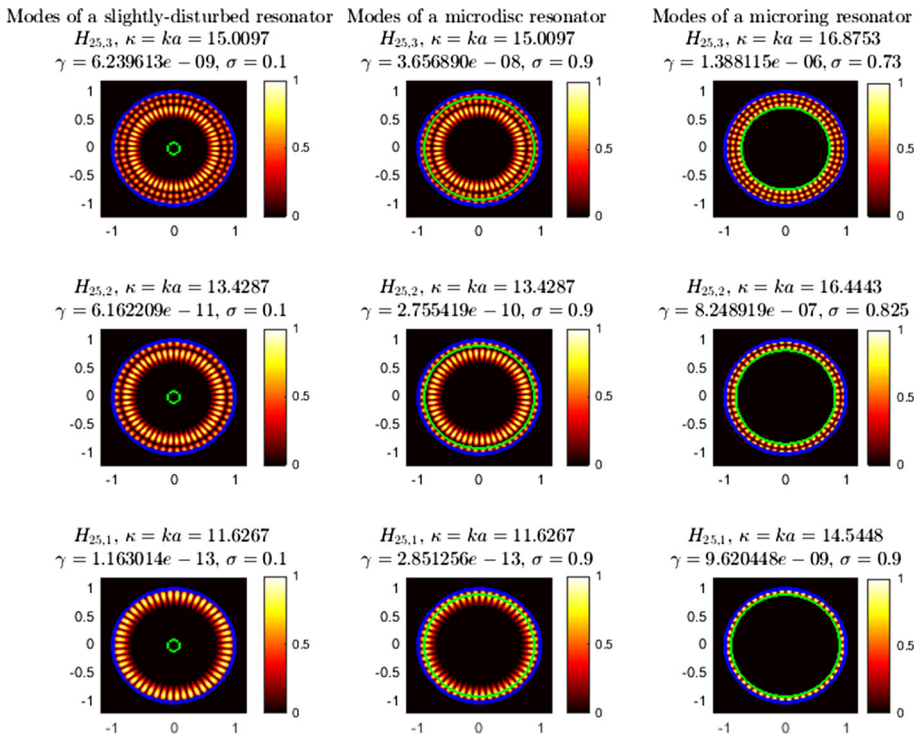
Fig. 5 Near fields of the H_{25,n} modes for n = 1, 2, 3 of slightly-disturbed microresonators (left column), microdisk resonators with the ring active region having \sigma = 0.9 (central column), and microring resonators with some values of \sigma corresponding to stable calculations (right column)
