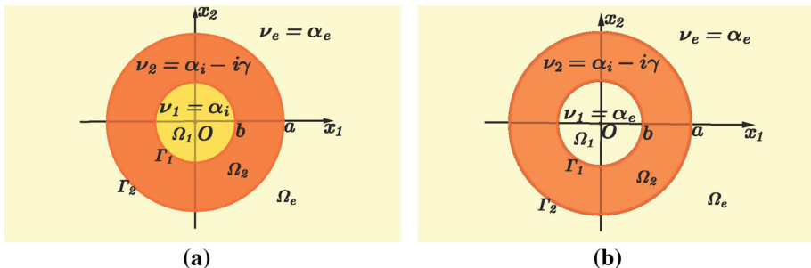
Fig. 1 Geometry of a microdisk with a ring gain area (a) and an active microring (b)
