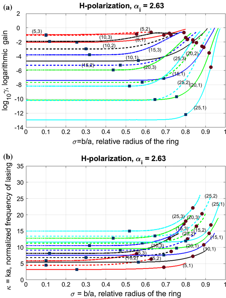
Fig. 4 Dependences of the threshold gains (a) and normalized frequencies of lasing (b) for the H-polarized WG modes of a microring resonator on the radii ratio \sigma
