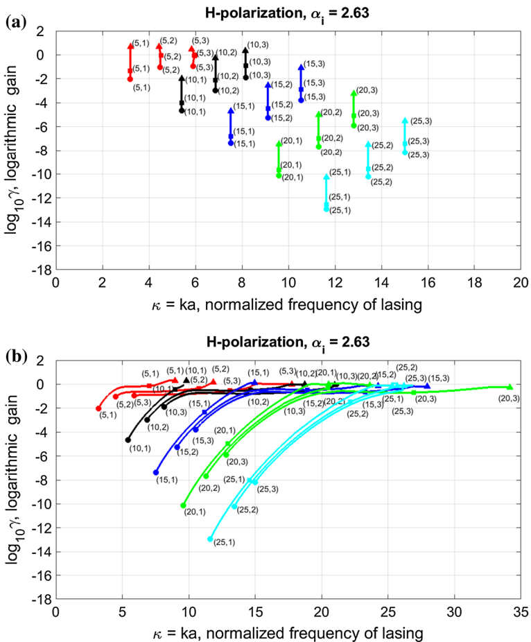
Fig. 2 Normalized frequencies of lasing and threshold gains for the H-polarized modes of a microdisk resonator with a ring gain area (a) and a microring resonator (b) . Eigenvalues for the relative radius of the ring \sigma = b/a = 0 are marked by circles, for \sigma = 0.9 by squares, and for \sigma = 0.999 by triangles
