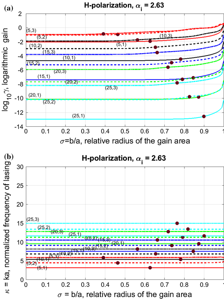
Fig. 3 Dependences of the threshold gains (a) and normalized frequencies of lasing (b) for the H-polarized WG modes of a microdisk resonator with a ring gain area on the radii ratio \sigma
