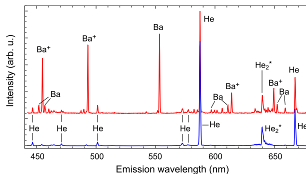
FIG. 6. Typical emission spectra of He-Ba r.f. plasma above a free surface of superfluid He. T = 1.65 K, f_{dis} = 5 Hz, \tau_{dis} = 50 \mu\text{s} , r.f. power 190 W. Upper (red) curve - ablation laser on, lower (blue) curve - ablation laser off.
