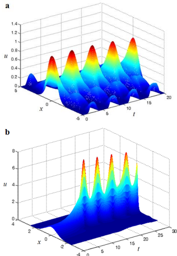
Fig. 3. Evolution of a Gaussian soliton-like envelop pulse in nonstationary medium at \alpha, f' = 0 : a) \beta = 0.5, \gamma = -1+0.01\sin 2\pi t ; b) \gamma = -1, \beta(t) = -0.5 for t \leq 5 and \beta(t) = 0.5(1+0.2\sin 2\pi t) for t > 5 ; the cases of negative nonlinearity.
