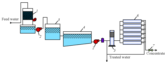
Figure 1. A flow diagram of a ground water treatment system using reverse osmosis: 1 - aeration column; 2 - booster pump; 3 - rapid sand filter; 4 - pure water tank; 5 - working pump of reverse osmosis facility; 7 - pressure regulation valve;
