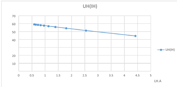
Figure 2. External characteristic
