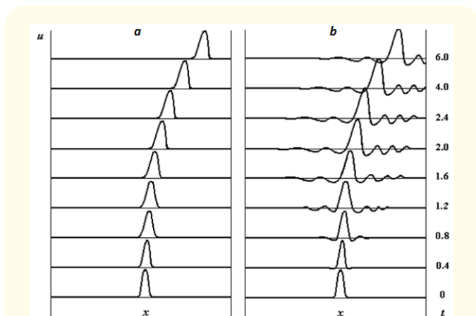
Figure 2: Evolution of pulse (2) with \alpha=1 , \beta=2.3 \cdot 10^{-3} , v=0.01 at its propagation in a fiber: (a) \gamma=0 , (b) \gamma=1 \cdot 10^{-4} .
