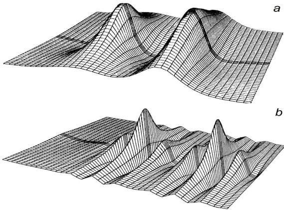
Fig. 3. Formation of the 2D bi-soliton at u_1(0)=1.35 , u_2(0)=1.3 , \Delta x(0)=6 : (a) t=0 ; (b) t=0.9 .
