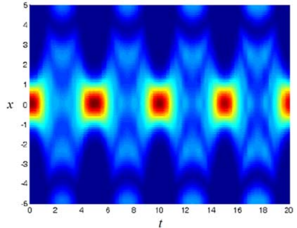
Fig. 5. Evolution of a 1D Gaussian envelop pulse in nonstationary medium at \beta = 0.5 , \gamma = -1+0.01\sin 2\pi t .
