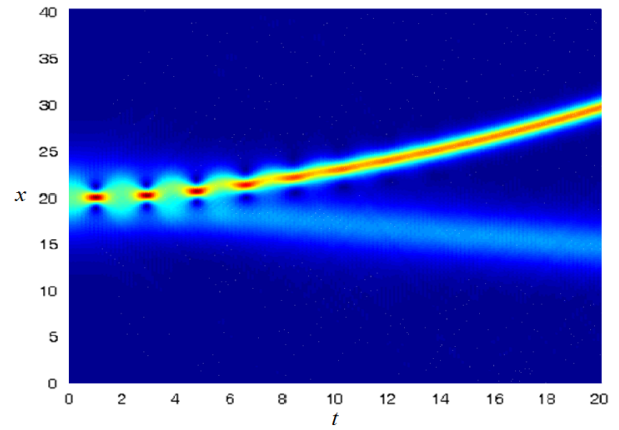
Fig. 4. Evolution of a 1D Gaussian envelop pulse in nonstationary medium at \beta(t) = -0.5(1+\sin 0.1\pi t) , \gamma = -1 .
