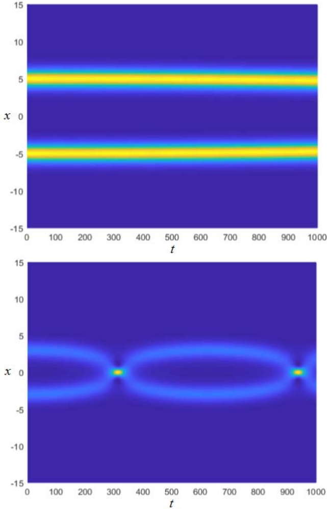
Fig. 6. Interaction of two pulses u_0 = A[\text{sch}(x-s/2) + \text{sch}(x+s/2)] , A = \sqrt{|\beta/\gamma|} in stationary medium for \beta = 0.05 , \gamma = -1 ; \alpha, f' = 0 ; s = 10, 5 .
