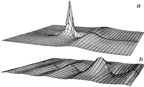
Fig. 2. Formation of the 2D soliton with oscillating structure at interaction initial pulses u_1(0)=8 , u_2(0)=1 at \Delta x(0)=4 : (a) t=0 ; (b) t=0.8 .
