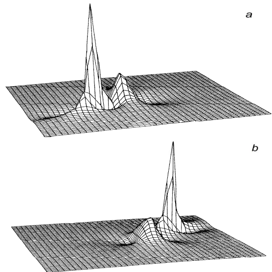
Fig. 1. Collision of the 2D solitons with algebraic asymptotics at u_1(0)=12, u_2(0)=4, \Delta r(0)=3.3 : (a) t=0 ; (b) t=0.7 .
