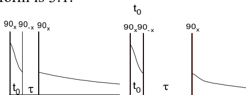
Fig.1. The effect of the Goldman-Schen pulse sequence at two different times of mixing \tau .
