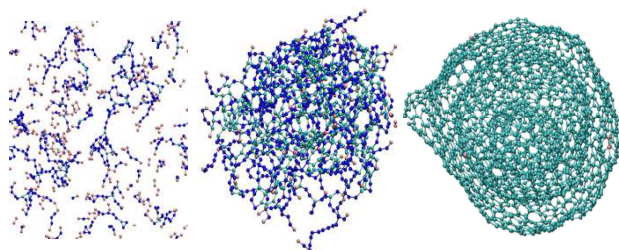
Fig.1. The stages of the fullerene formation
