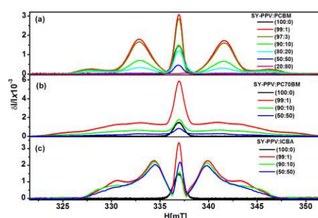
Fig. 1: EDMR of fullerene TEs in blends with a donor polymer, demonstrating efficient population after photoinduced charge transfer. [1]
