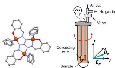
Fig.1. Left: the molecular structure of the spin-frustrated \text{Cu}_3 , with a ground state S=1/2 . Right: schematic view of the modified version of the sample holder used for the EFM-EPR measurements.
