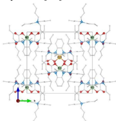
Fig.1 a/b/c projection of VASP optimized CuI in Ni-polymorphs matrix
