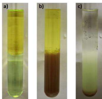
Figure. 2-phase system consisting of cyclohexane/methanol containing 1 , CuSO 4 and styrene. a) Parent mixture; b) Cu nanoparticles after 120 s of irradiation of the bottom methanol solution c) After subsequent irradiation (120 s) of the upper cyclohexane phase. The milky precipitate is polystyrene.
