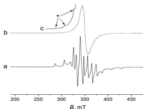
Fig.2. EPR spectra of \text{V}_2\text{O}_5 (a) and \text{V}_2\text{O}_5/\text{BTA} (b) at 77 K. Spectra are normalized by the amplitude. c is fivefold enlarged part of b , arrows show the lines of the spectrum a .
