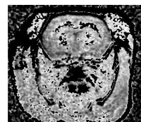
Fig. 2. MPF map of the rat brain.
