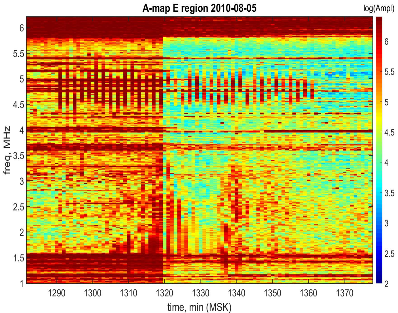
Fig. 2. Enlarged fragment of the A-map of the ionosphere E region.
