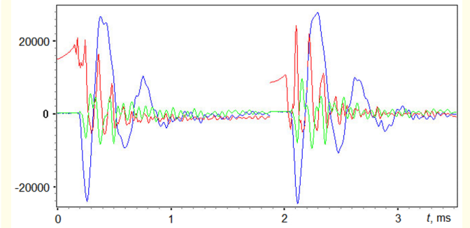
Figure 8: Oscillograms of two impacts on a granite sample: red line - the electrical signal, blue and green lines - two seismic components.
