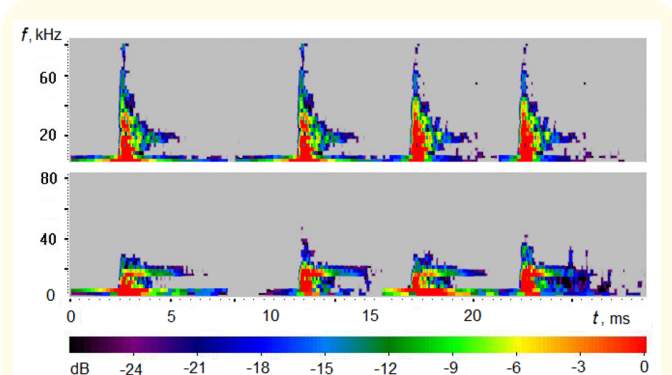
Figure 9: Spectrograms of the impacts on a granite sample corresponding to the oscillograms shown in figure 8.
