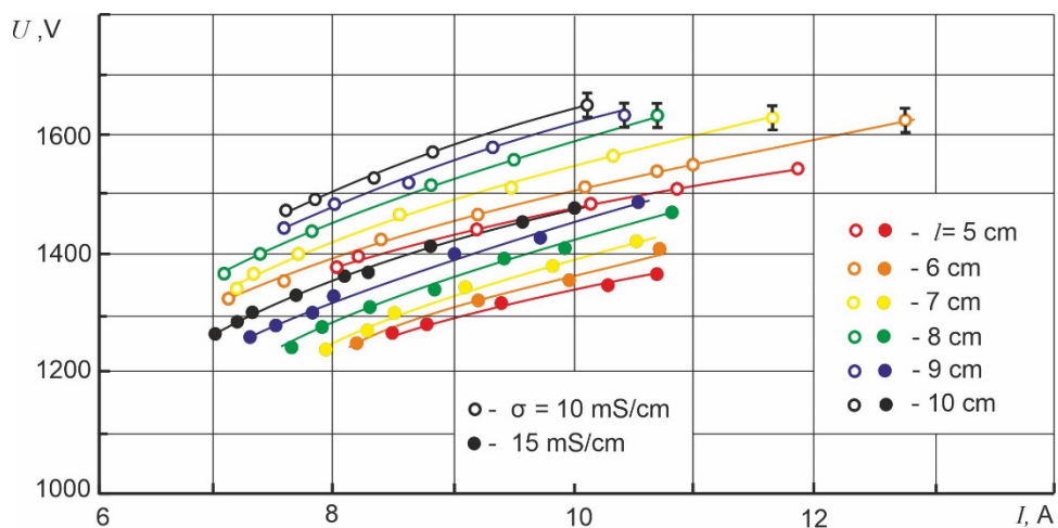
Fig. 2. Current-voltage characteristics.
