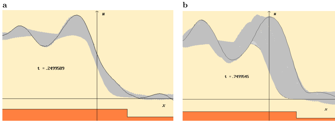
Fig. 5. Evolution of "step" (9) in the model (10) with c < 0 : a - t \approx 0.25 ; b - t \approx 0.75
