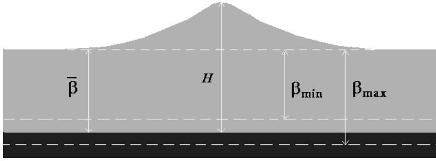
Fig. 2. Dependence \beta = \beta(t, x) of type of “bottom oscillations”, models (12)
