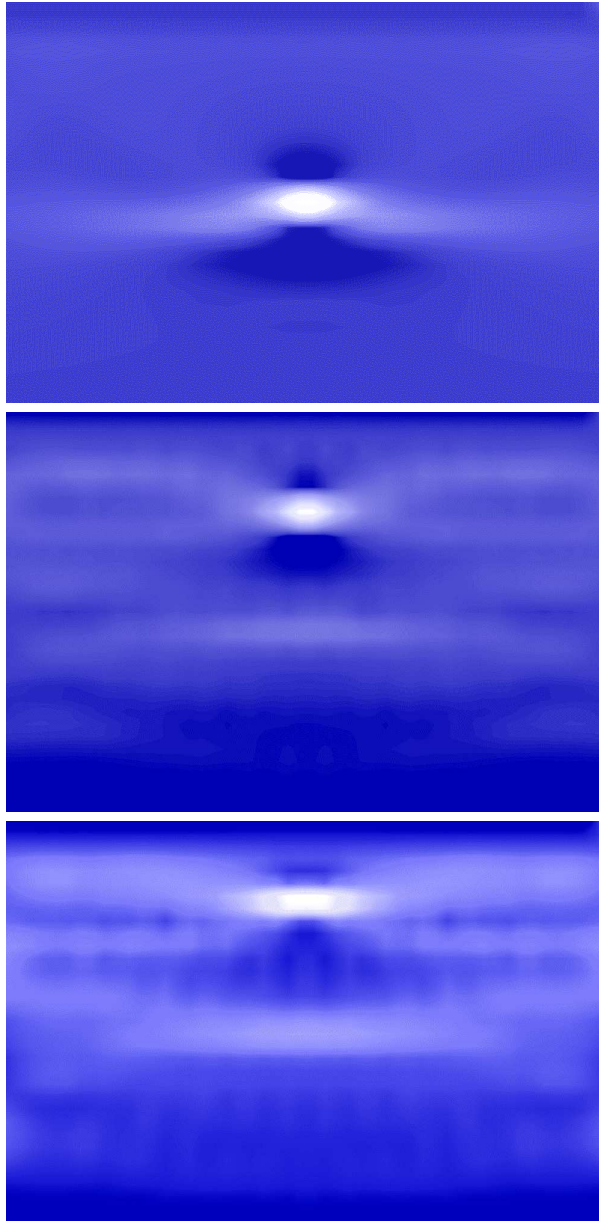
Fig. 9. Evolution of 2D soliton of eq. (13) at t = 0.4, 1.2, 2.0 .
