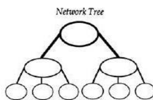
Figure 2. Network Tree
