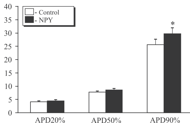
Fig. 2. APD20%, APD50%, and APD90% in the preparations of rat right atrium in control and upon exposure to 10^{-6} M of NPY. * p < 0.05 in comparison with the control.
