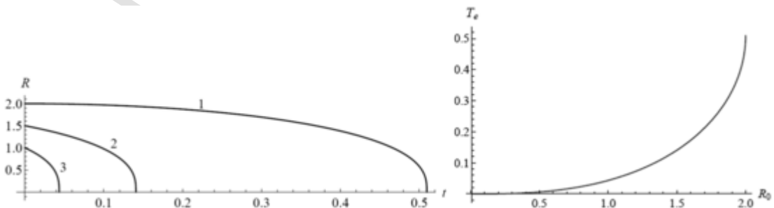
Fig. 4. Shrinking radius R(t) of a ponded spheroid for b = 2 , c = 1 , e = 0.1 , and R_0 = 2, 1.5, 1 (left panel, curves 1-3, respectively); extinction time for a spheroidal pond at b = 2 , c = 1 , and e = 0.1 (right panel).
