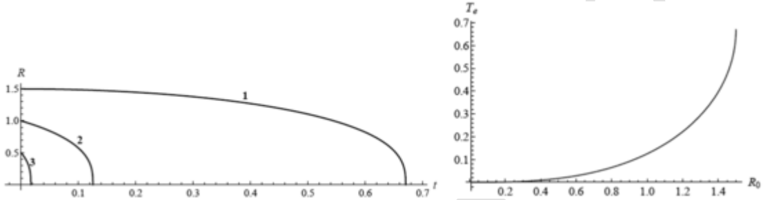
Fig. 3. Shrinking radius of the disk R(t) of a ponded spherical cap for R_s = 1.5 , e = 0.1 , and R_0 = 1.5, 1, 0.5 (curves 1, 2, 3, respectively, left panel); extinction time T_e(R_0) for ponds made by a spherical cap having R_s = 1.5 ; surface water is subject to evaporation e = 1 (right panel).
