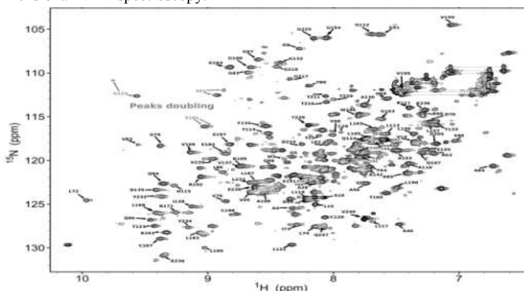
Fig. 1. 1 H, 15 N-HSQC spectrum of 15 N-WBSCR27, recorded at 600 MHz in 90% 2 H 2 O/10% D 2 O
