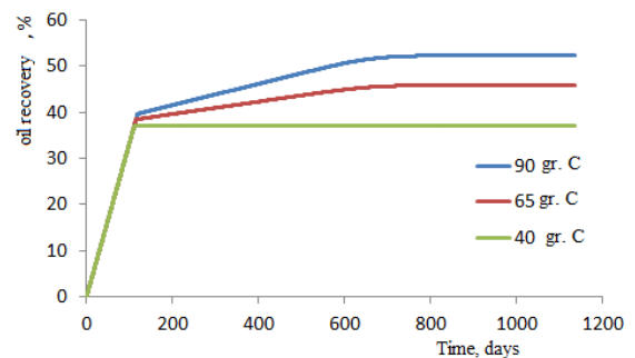
Fig. 5. Calculated oil recovery (oil 1).
