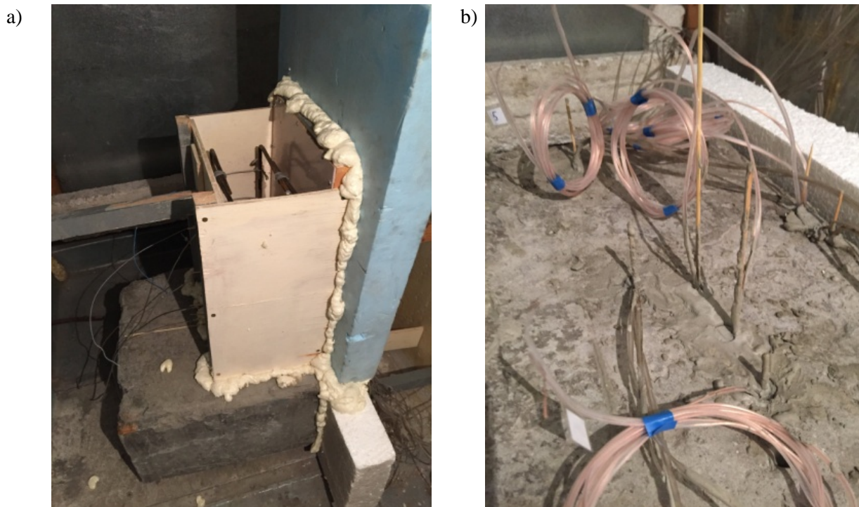
Fig. 1. Experimental design a - general view, b - the process of installing sensors.
