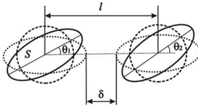
Figure 2. Illustration to definition of the initial state parameters of vortex system
