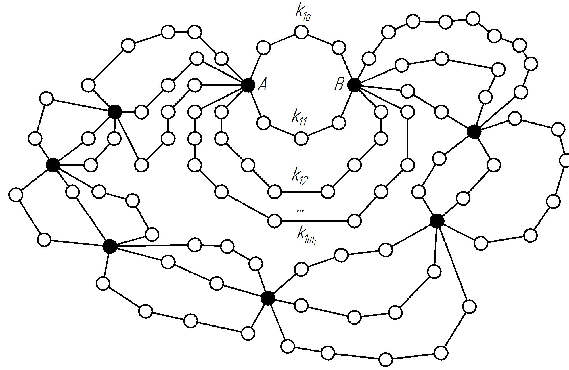
Fig. 2. A ring of t “necklaces”. For this graph, t = 8 and m_i = 2 for i = 2, \dots, 8 . Sources and a sinks are bolded
