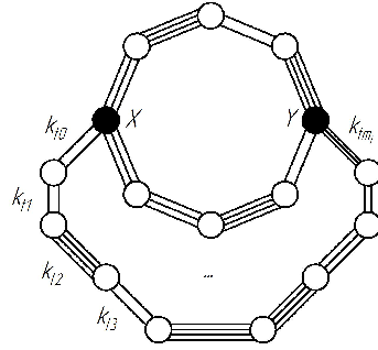
Fig. 4. The multigraph dual to the ring of necklaces graph with t = 3
