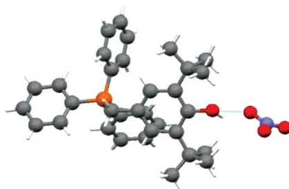
Figure 2 Structure of 6. (Color figure available online).
