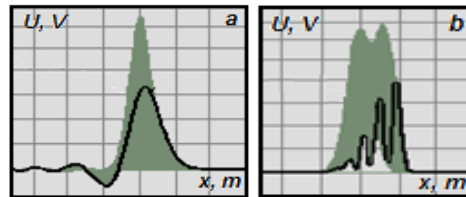
Figure 1: Evolution of a pulse: a) dispersion effect, b) formation of soliton-like structures.
