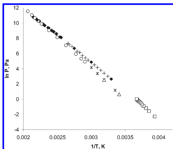
Figure 1. Experimental vapor pressures of formamide: ●, ref 12; ■, ref 9; ○, ref 8; △, ref 10; □, ref 13; *, ref 11; ×, this work.
