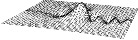
Fig. 5. Evolution of 2D soliton: v=1 , \beta<0 , \gamma>0 : t=0.2 .
