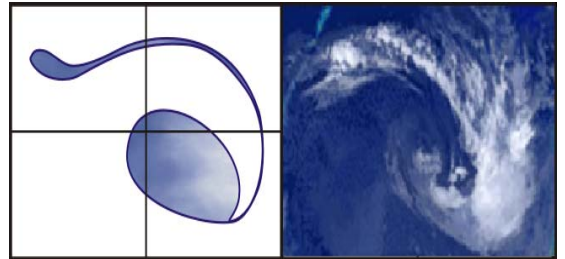
Fig. 9. Simulation of evolution of the cyclonic type synoptic vortex (numerical result and satellite photo).
