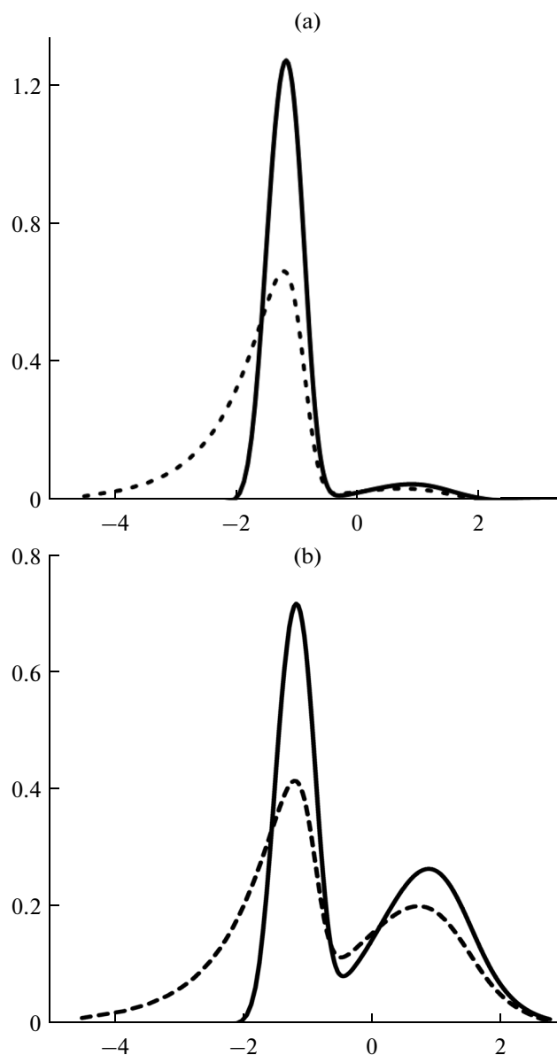
Fig. 5. The coercivity spectra obtained from the isothermal curves of magnetization (the solid line) and remagnetization (the dashed line) for the parameters of DF indicated in Fig. 4: (a) c = 0.1 ; (b) c = 0.5 . Here, c is the relative contribution of the population of the SD grains in the total remanent magnetization. Correspondingly, the contribution of the MD grains is 1 - c .
