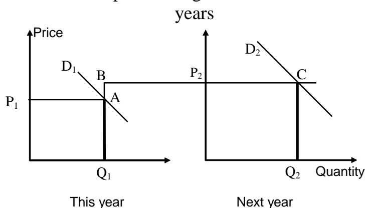
Figure 4. Rule of effective price-fixing of a non-renewable resource for two years
