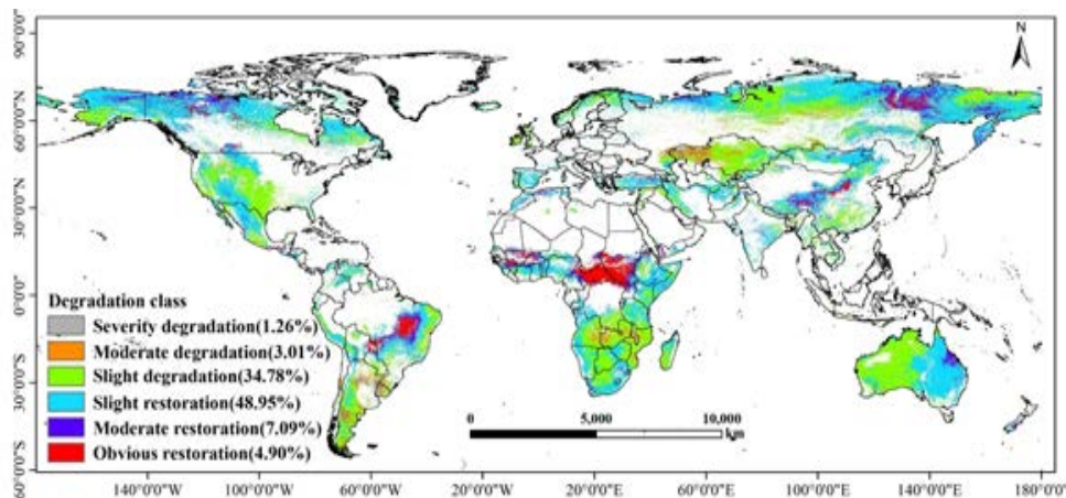
Fig. 1. Dynamics of grassland degradation or restoration across the globe from 2000 to 2013.
