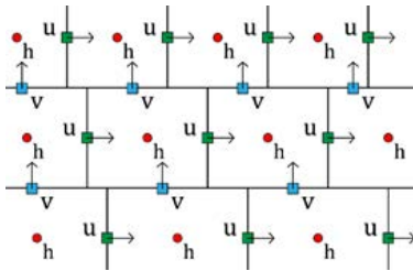
Picture 1. Staggered reduced grid variables placing schematic
