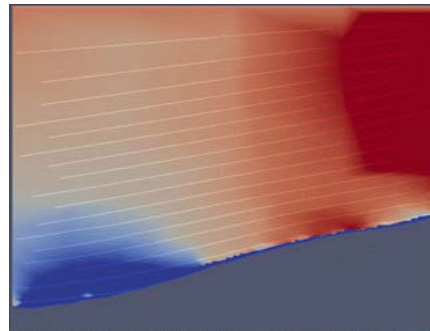
Figure 4. The dependence of the value of shear velocity from a point up the windward slope. The results of numerical simulation.
