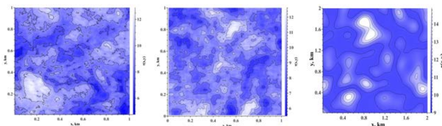
Fig. 2. The measured field of stratus optical thickness (on the left), numerical realizations of stratus optical thickness by methods (1), (3) (in the center) and by methods (2), (4) (on the right).
