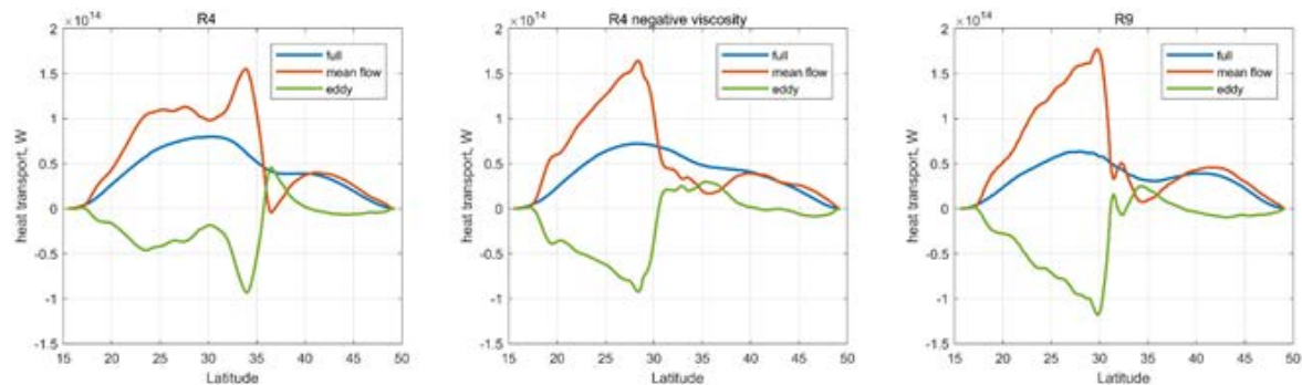
Figure 1. 20-years mean meridional heat flux in eddy-permitting (R4, R4 negative viscosity) and eddy-resolving (R9) models, in Watts. Total heat flux (full) is a sum of mean flow flux and eddy flux.
