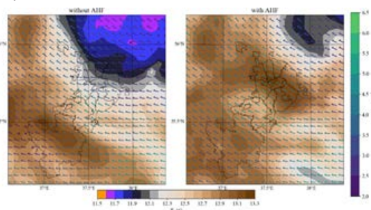
Fig. 3. Results of temperature and wind fields modeling (without AHF – left, with AHF – right).
