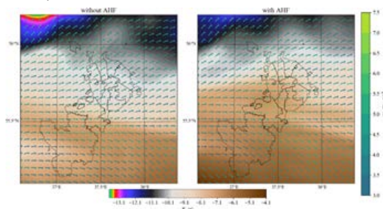
Fig. 3. Results of temperature and wind fields modeling (without AHF – left, with AHF – right).
