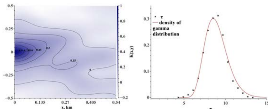
Fig. 1. Autocorrelation function K(x, y) (on the left) and one-dimensional distribution density of the cloud optical thickness field (on the right).
