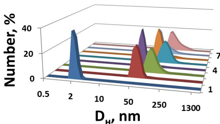
Figure 6. Number-averaged size distribution for the IA-12/oNu binary system at various amphiphile/oNu molar ratios: 1—individual oNu, 2—0.02, 3—0.045, 4—0.094, 5—0.194, 6—0.394, 7—0.79, 8—1.2; 9—3.9; 25 °C.
