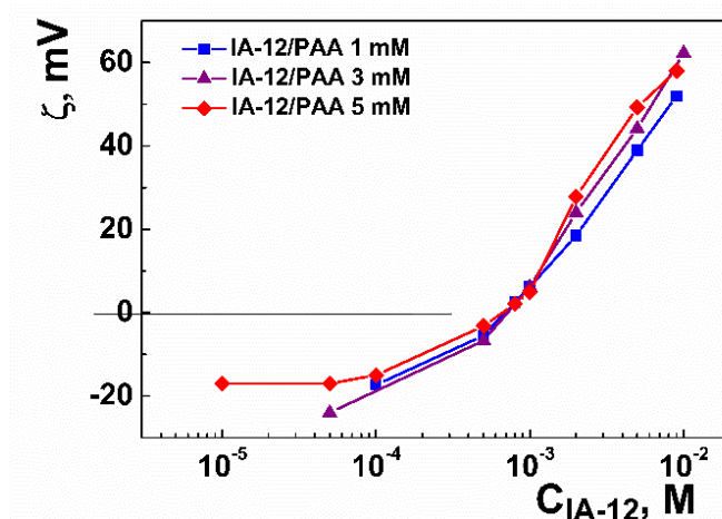
Figure 4. Zeta potential versus IA-12 concentration plot for the IA-12/PAA binary systems; 25 °C.
