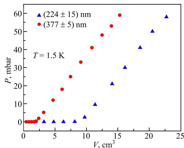
FIG. 3. Adsorption isotherms of ^3\text{He} on the surface of inverse opal \text{SiO}_2 samples, at a temperature of 1.5 K.
