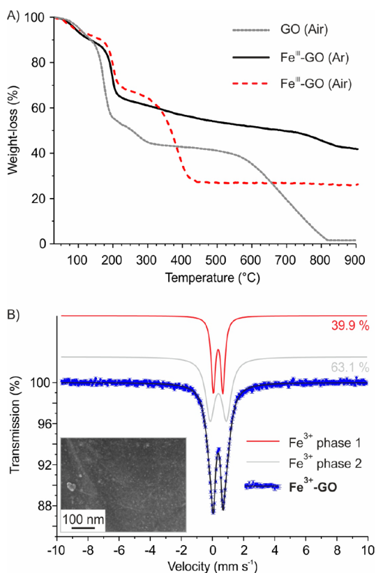
Figure 2. \text{Fe}^{3+} -GO characteristics. (A) TGA data in Ar and synthetic air, and comparison to GO. (B) Mössbauer spectrum (dotted blue line) and deconvolution into two components (red and light-gray lines). The inset of panel B is the SEM image of \text{Fe}^{3+} -GO.
